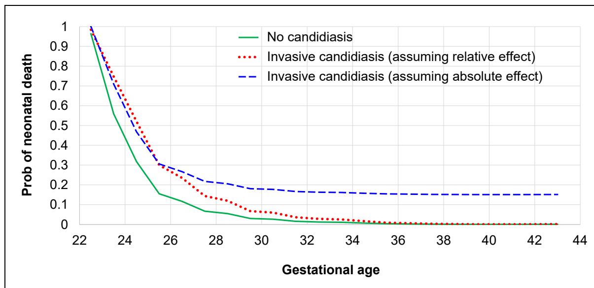
Figure HE007: Probability of death with and without invasive candidiasis
