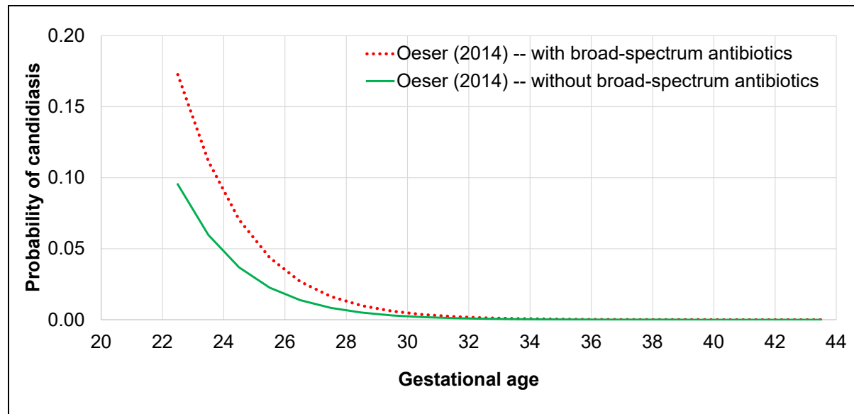
Figure HE004: Baseline risk of infection according to gestational age and exposure to broad-spectrum antibiotics, fitted to UK-specific incidence data
